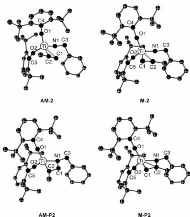
Figure 2. Optimized structures for the \pi complexes and the cycloaddition products with 2,6-di- tert -butylphenoxo ligand 1' (hydrogen atoms are omitted for clarity).
