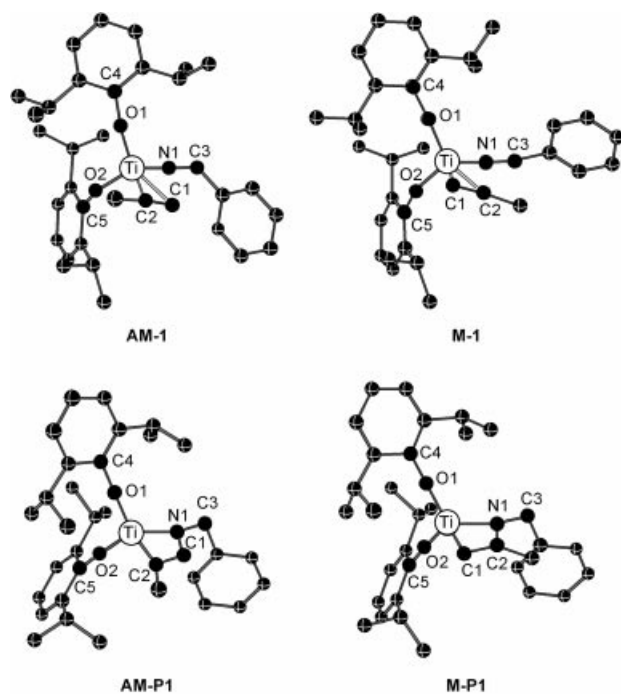
Figure 1. Optimized structures for the \pi complexes and the cycloaddition products with 2,6-diisopropylphenoxo ligand 8' (hydrogen atoms are omitted for clarity).
