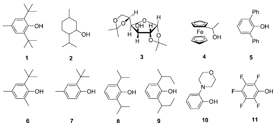
Scheme 2. Alkoxo and aryloxo monodentate ligands used in our study.
