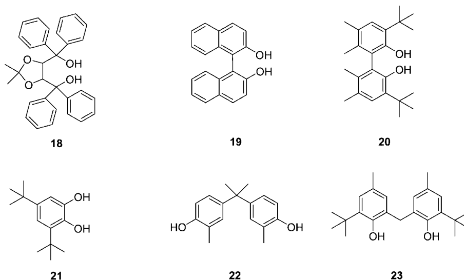
Scheme 3. Bidentate alkoxo and aryloxo ligands used in catalytic hydroamination reactions.
