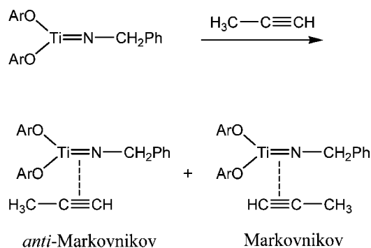
Scheme 4. anti -Markovnikov and Markovnikov coordination of propyne.
