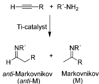
Scheme 1. Hydroamination of terminal alkynes.
